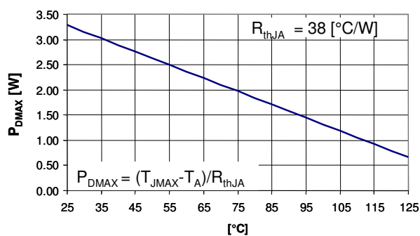
Figure 16. Maximum power dissipation vs T_A for DFN8 3x3 mm
