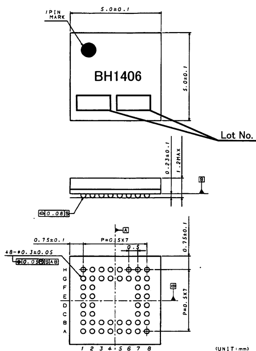
VBGA048T050 (Unit: mm)
