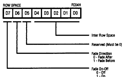
Figure 63. OSD Row Space Register (Write Only)
