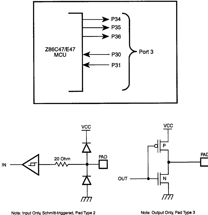
Figure 4. Port 3 Configuration
