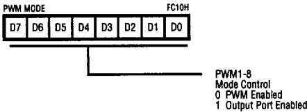
Figure 57. PWM Mode Register (Write Only)
