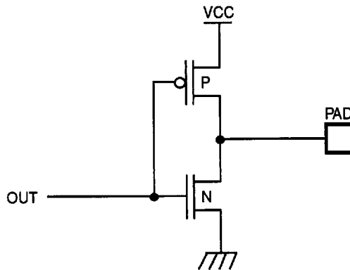
Figure 6. Port 5 Configuration
