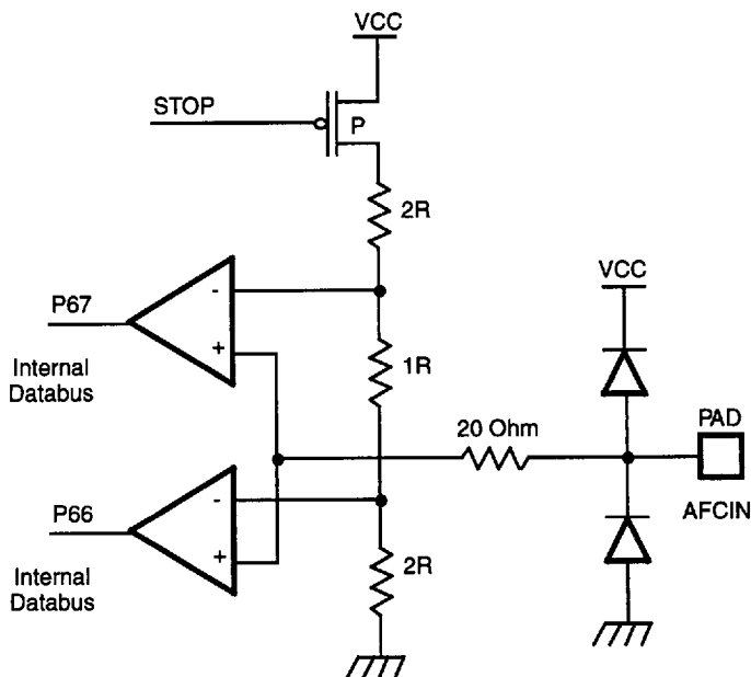
Figure 8. AFC IN Comparator Circuits
