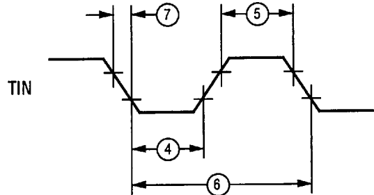
Figure 24. Counter Timer
