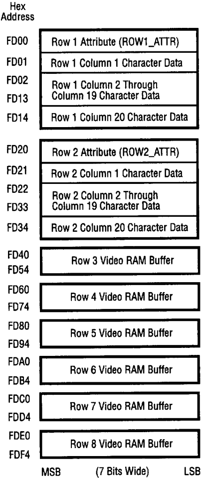
Figure 12. Video RAM Configuration
