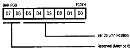
Figure 66. OSD Bar Position Register (Write Only)
