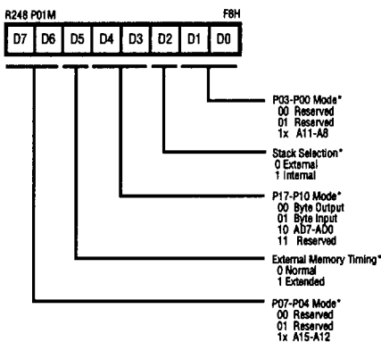
Figure 76. Port 0 and 1 Mode Register (F8H; Write Only) *(For Z86E47 only)
