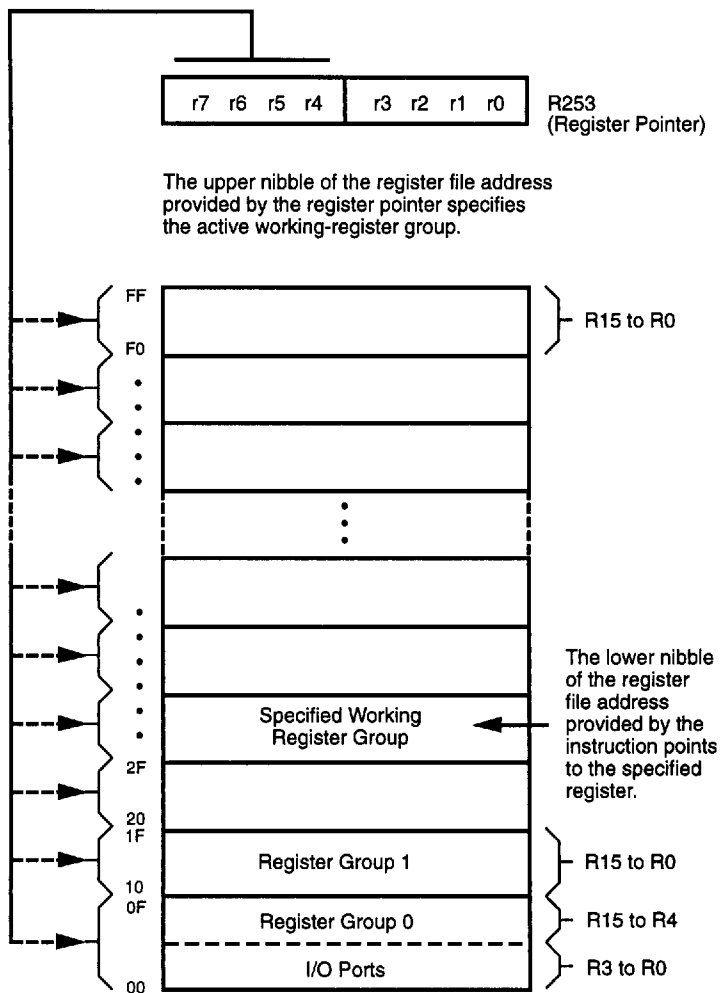
Figure 16. Register Pointer
