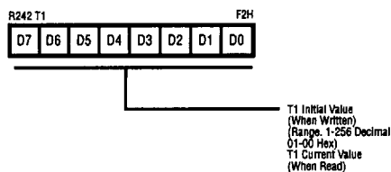
Figure 70. Counter Timer 1 Register (F2H; Read/Write)
