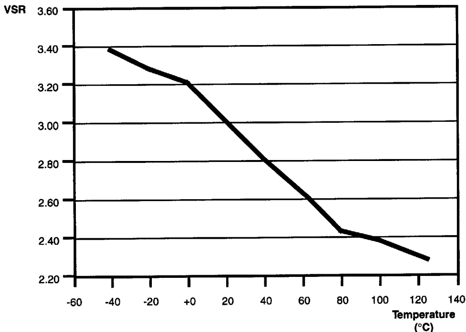
Figure 21. Typical Voltage Sensitive Reset vs Temperature
