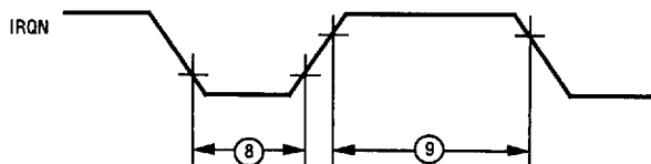
Figure 25. Interrupt Request
