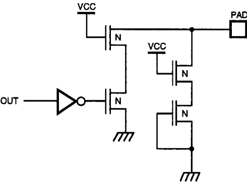
Figure 34. Output Only, 12-Volt Open-Drain (Pad Type 7)
