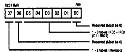
Figure 79. Interrupt Mask Register (FBH; Read/Write)
