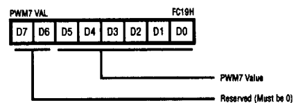
Figure 50. PWM 7 Value (Write Only)
