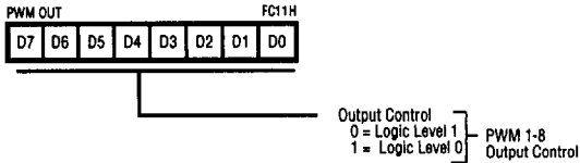
Figure 58. PWM Port Output Register (Write Only)
