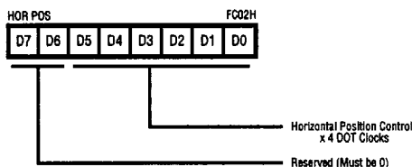
Figure 61. OSD Horizontal Position Register (Write Only)
