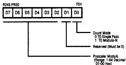
Figure 73. Prescaler 0 Register (F5H; Write Only)
