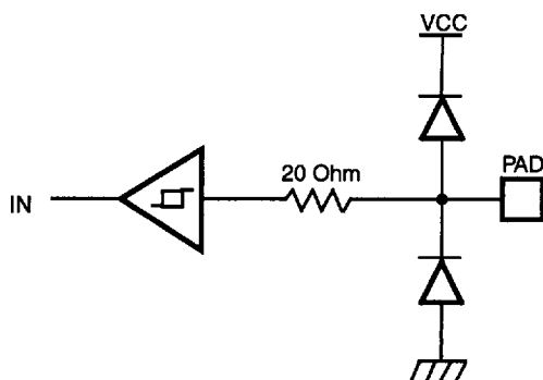
Figure 7. Port 6 Configuration
