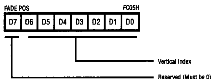
Figure 64. OSD Fade Position Register (Write Only)
