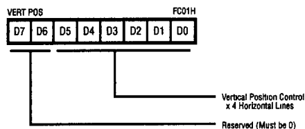
Figure 60. OSD Vertical Position Register (Write Only)
