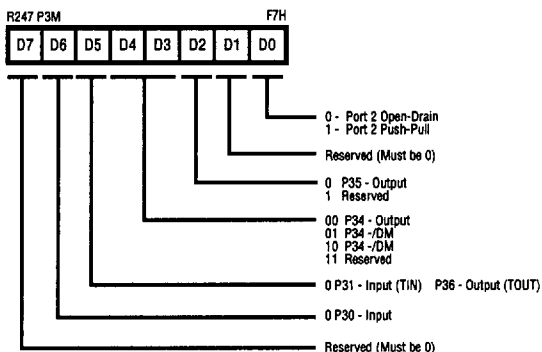
Figure 75. Port 3 Mode Register (F7H; Write Only)
