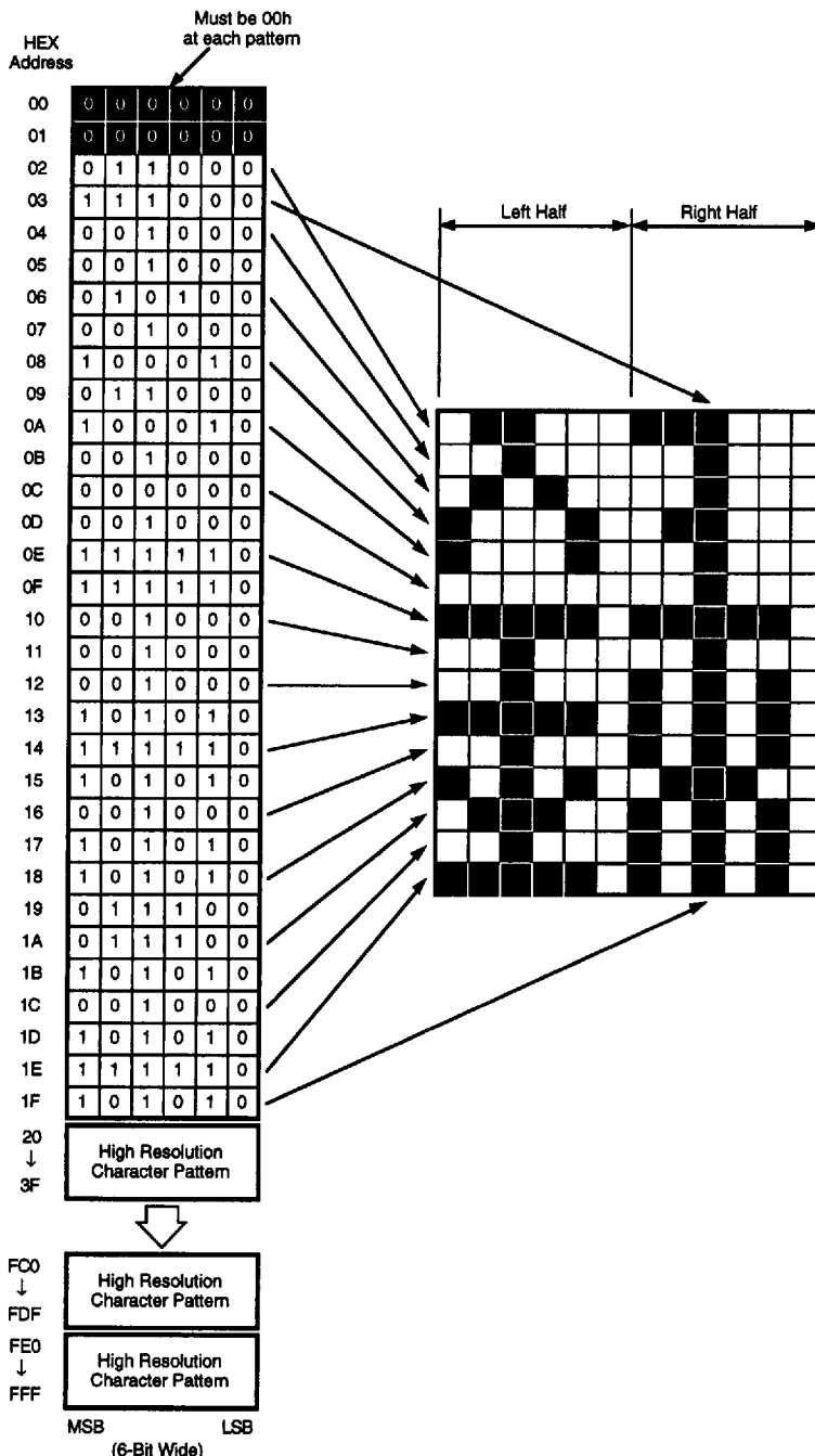
Figure 11. Character ROM Configuration
