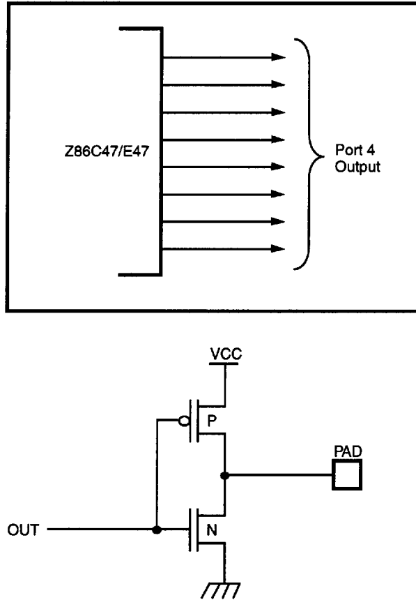
Figure 5. Port 4 Configuration
