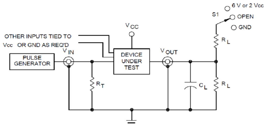
Figure 5. Test circuit
