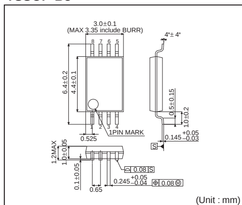
TSSOP-B8
