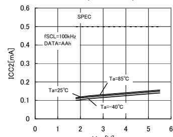
Fig.14 Current consumption at READ action ICC2 ( f_{SCL} = 100\text{kHz} )
