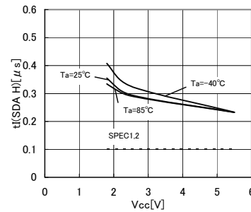
Fig.31 Noise removal valid time t_I(\text{SDA H})
