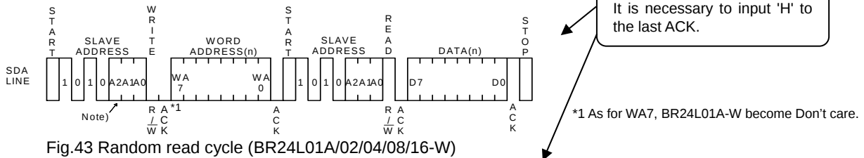
Fig.43 Random read cycle (BR24L01A/02/04/08/16-W)
