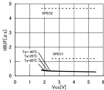
Fig.27 Bus release time before transfer start t_{BUF}
