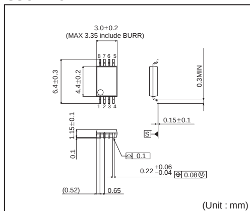
SSOP-B8
