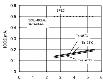
Fig.11 Current consumption at READ action ICC2 ( f_{SCL} = 400\text{kHz} )
