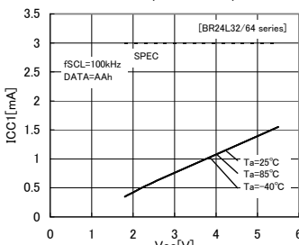
Fig.13 Current consumption at WRITE action ICC1 ( f_{SCL} = 100\text{kHz} )
