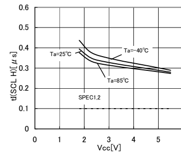
Fig.29 Noise removal valid time t_I(\text{SCL H})
