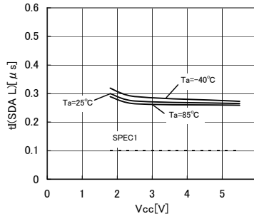
Fig.32 Noise removal valid time t_I(\text{SDA L})
