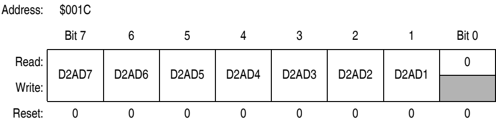
Figure 15-2. DDC2 Address Register (D2ADR)
