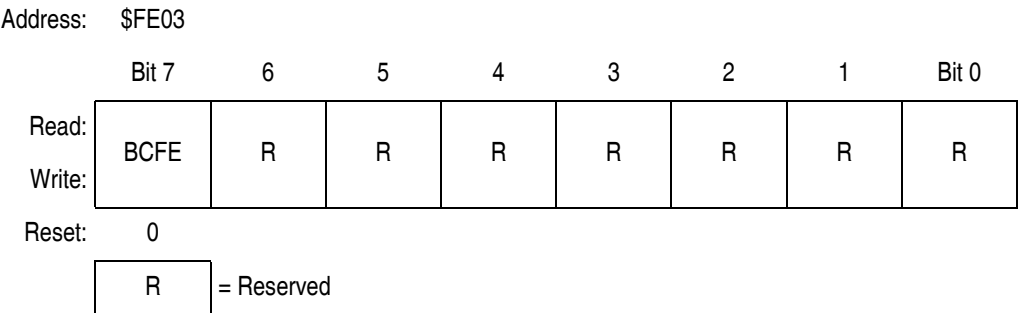
Figure 7-20. SIM Break Flag Control Register (SBFCR)
