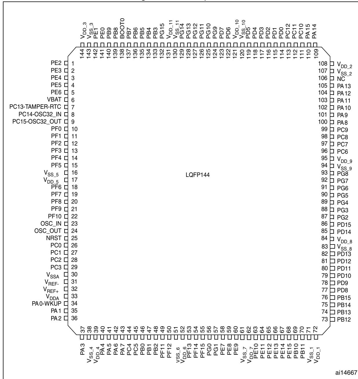
Figure 3. LQFP144 pinout
