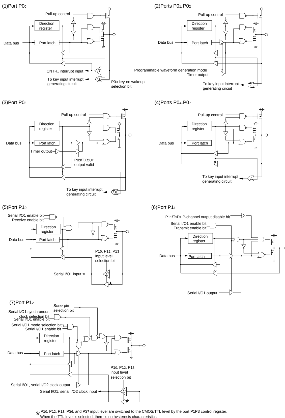
Fig. 17 Block diagram of ports (1)
