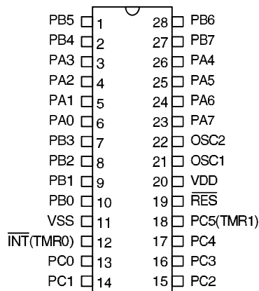
HT48C50 – 28 SKDIP-H
