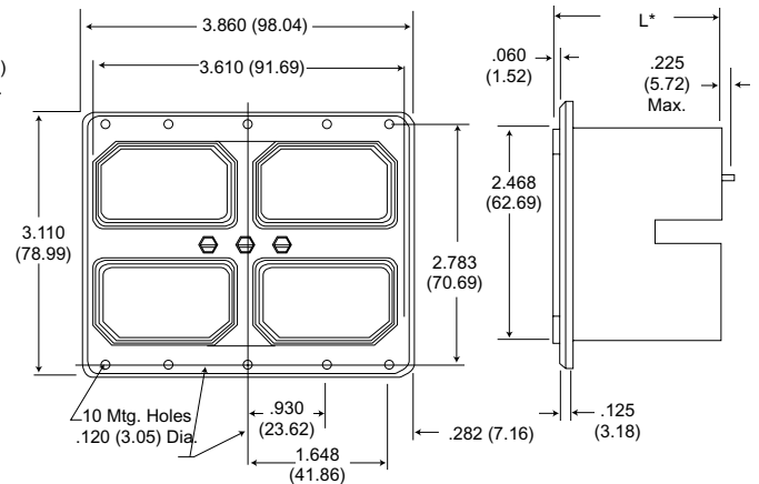
34 Shell
