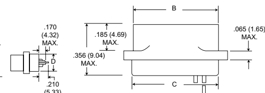
Solder Pot
