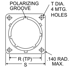
RECEPTACLE ASSEMBLY
