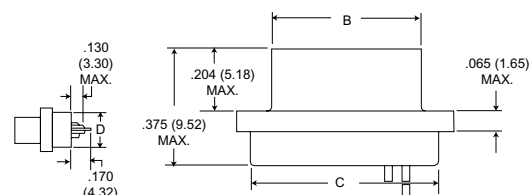
Solder Pot
