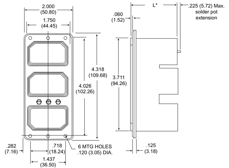
34 Shell
