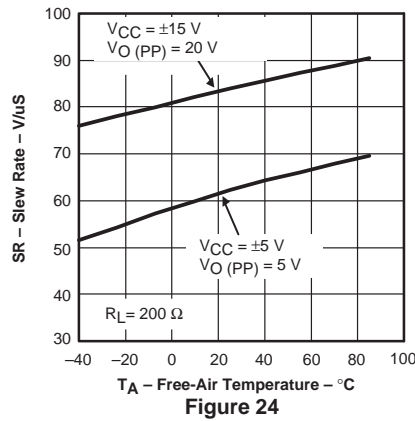
PREAMP SLEW RATE vs FREE-AIR TEMPERATURE
