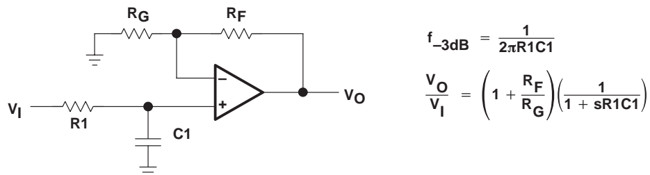
Figure 63. Single-Pole Low-Pass Filter
