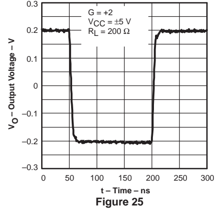
PREAMP 400-mV STEP RESPONSE
