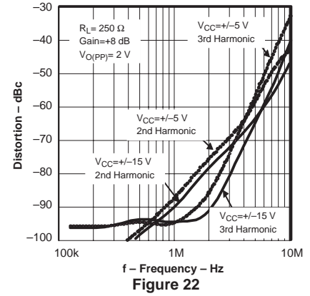
PREAMP HARMONIC DISTORTION vs FREQUENCY
