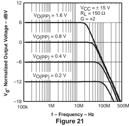
PREAMP LARGE AND SMALL SIGNAL FREQUENCY RESPONSE
