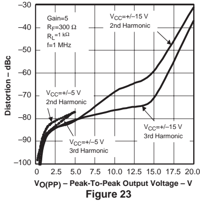
PREAMP HARMONIC DISTORTION vs OUTPUT VOLTAGE
