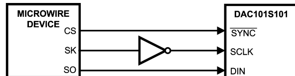
FIGURE 8. Microwire Interface
