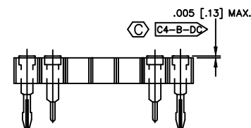
OPTION -L: REPLACE BOTH END POS. (BOTH ROWS) AS SHOWN FIGURE 4 (SEE NOTE 9 SHT.1)
