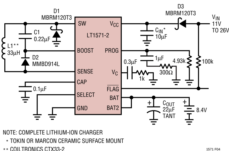
Figure 4. 200kHz Charging Lithium Batteries (Efficiency at 1A > 87%)
