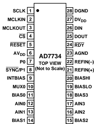
Figure 11. 28-Lead TSSOP
