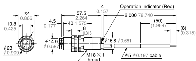
CY-29 Sensor
