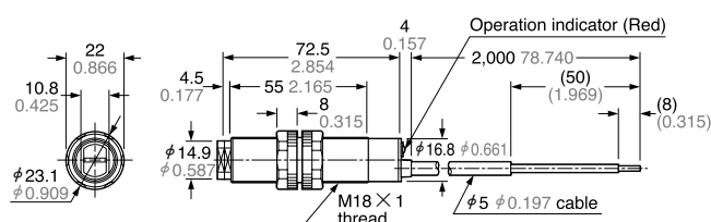
CY-19 Sensor
