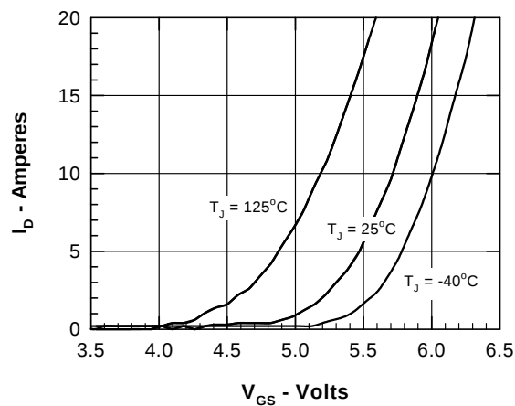
Fig. 6. Admittance Curves
