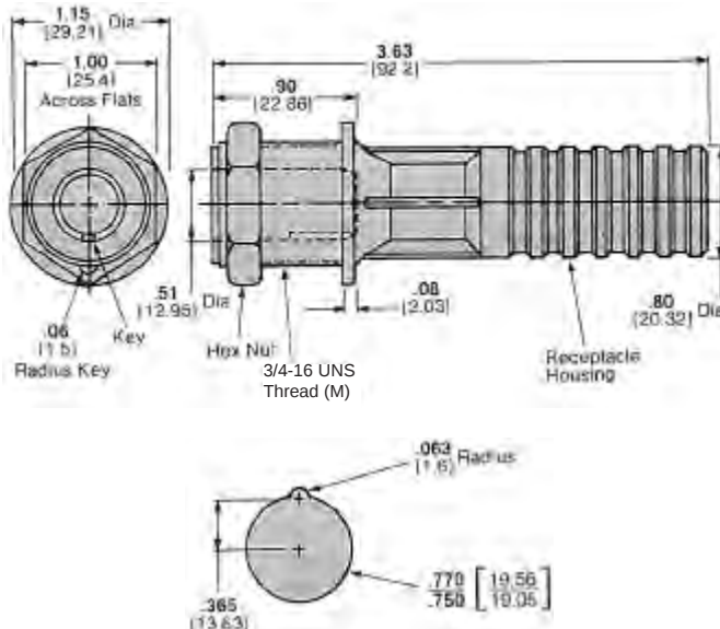
Recommended Panel Cutout for Bulkhead Mounting
