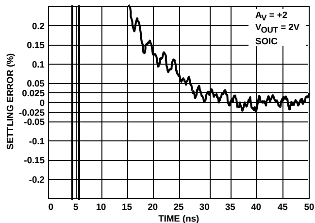
FIGURE 17. SETTLING RESPONSE
