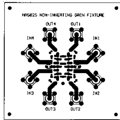
TOP LAYOUT
