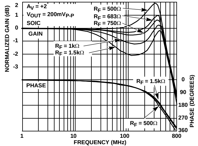
FIGURE 13. FREQUENCY RESPONSE vs FEEDBACK RESISTOR
