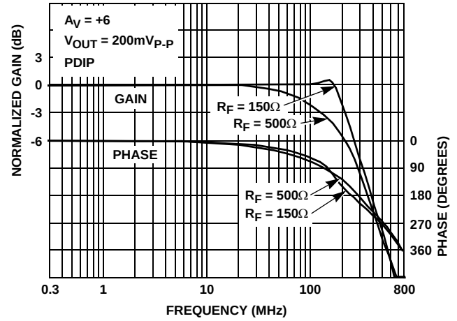
FIGURE 29. FREQUENCY RESPONSE
