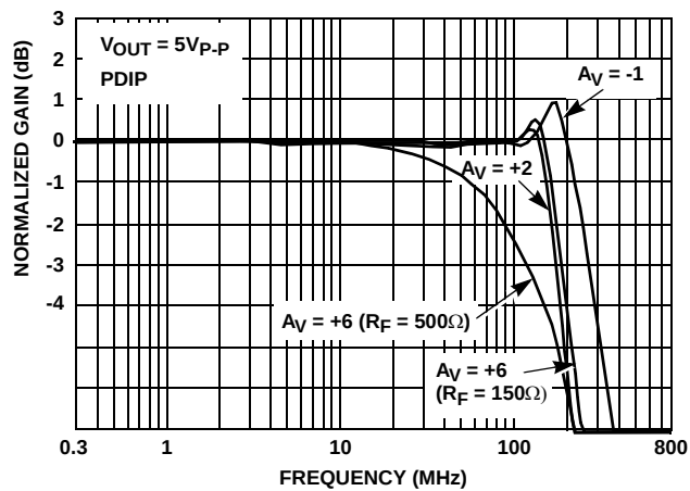
FIGURE 30. FULL POWER BANDWIDTH
