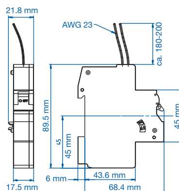
Dimensions UA120UM.
