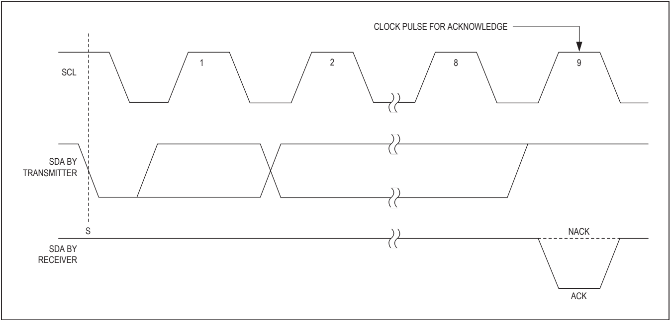
Figure 11. Acknowledge
