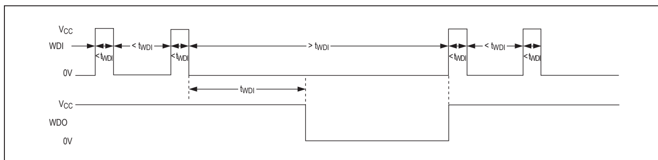
Figure 7. Watchdog Timer Operation
