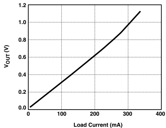
Figure 6. Dropout Voltage with Load Current
