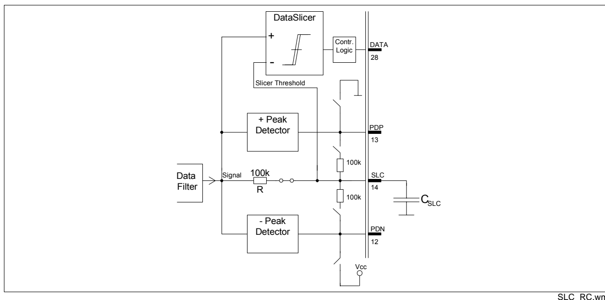
Figure 3-25 Slicer Level using RC Integrator
