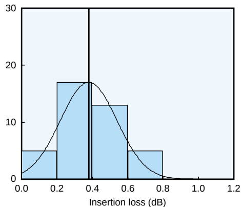
a) Insertion loss
