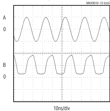
RESPONSE TO 50MHz \pm 10mV SINE WAVE
