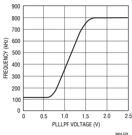
Figure 6. Relationship Between Oscillator Frequency and Voltage at the PLLLPF Pin When Synchronizing to an External Clock
