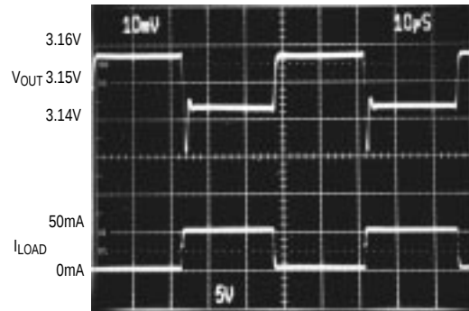
LOAD-TRANSIENT RESPONSE
