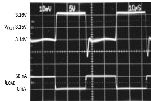
LOAD-TRANSIENT RESPONSE
