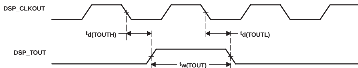
Figure 6–15. DSP_TOUT Timing
