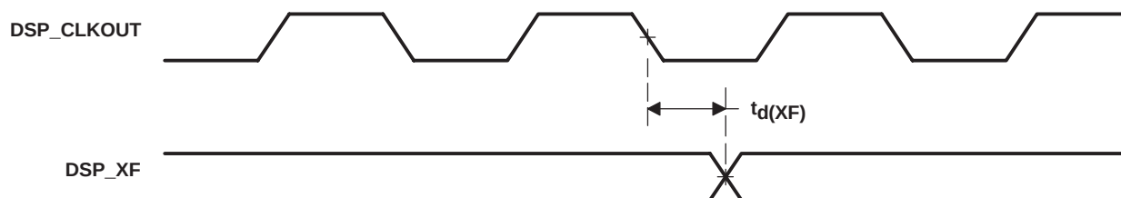
Figure 6–14. DSP_XF Timing
