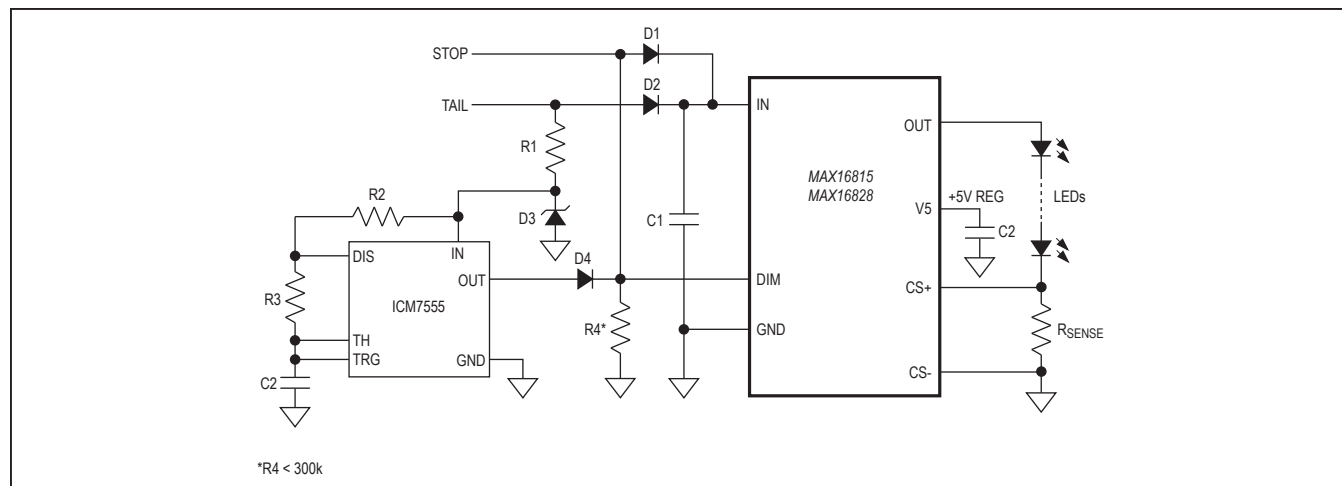
Figure 1. PWM Dimming Operation with ICM7555 Timer
