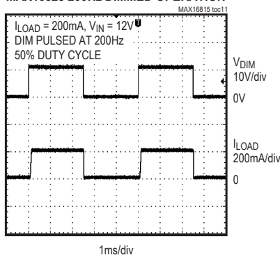
MAX16828 200Hz DIMMED OPERATION
