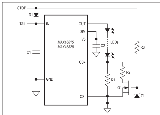
Figure 3. Two-Level Brightness with Current Level Switch for TAIL/STOP Lights
