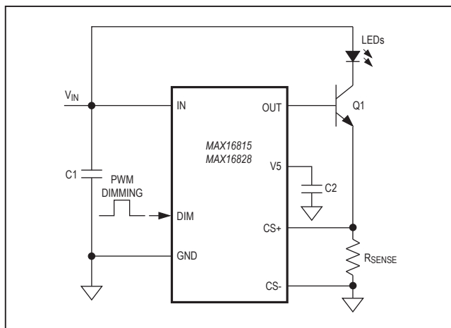
Figure 4. Increased LED Current (Ampere Range) with a Single BJT
