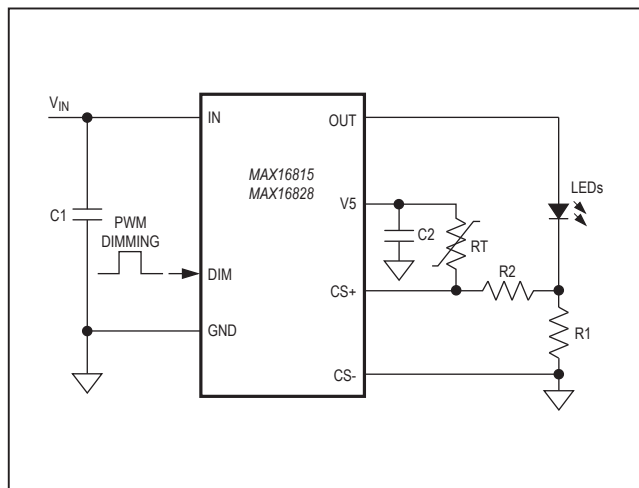
Figure 2. LED Current Thermal Foldback with an NTC Thermistor
