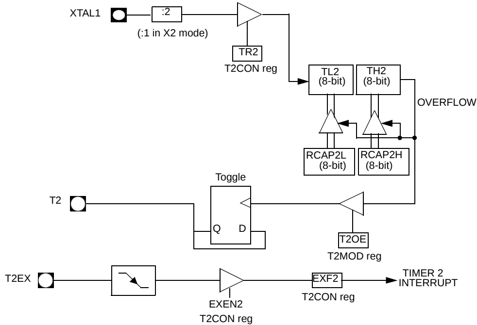
Figure 6-3. Clock-Out Mode \overline{C/T2} = 0
