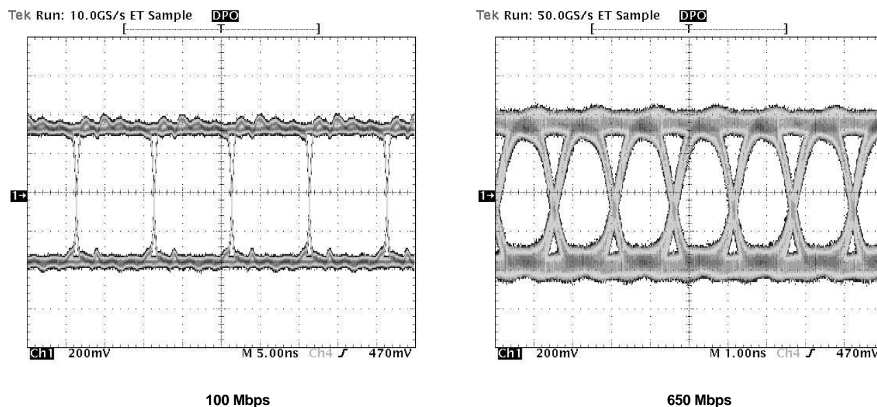
Figure 15. Typical Driver Eye Pattern for the SN65LVDM1676
