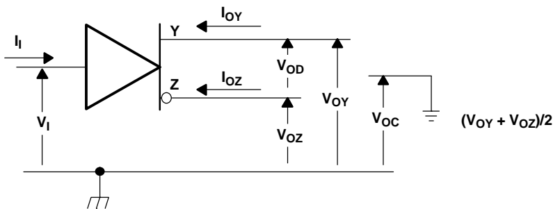
Figure 1. Driver Voltage and Current Definitions
