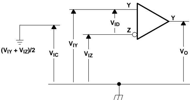
Figure 6. Voltage Definitions
