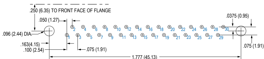
30 Pin
