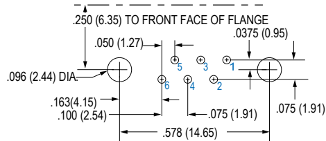
6 Pin
