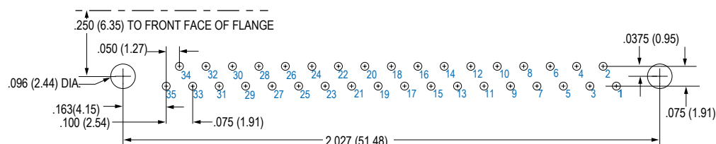
35 Pin
