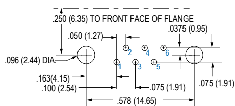
6 Pin
