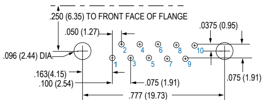
10 Pin
