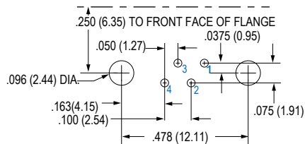
4 Pin
