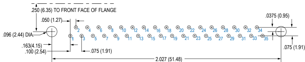
35 Pin
