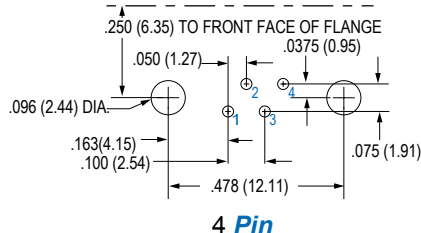
4 Pin
