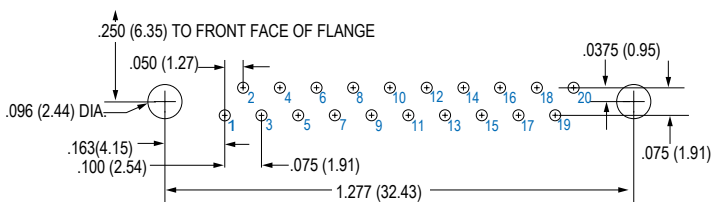
20 Pin
