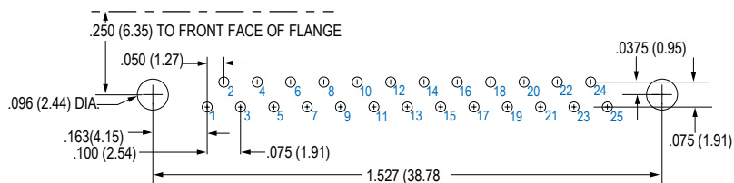
25 Pin
