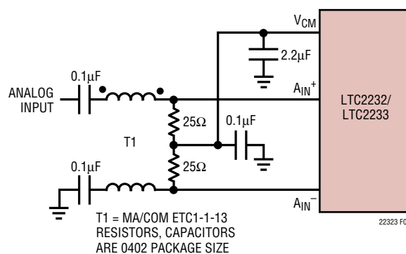
Figure 7. Recommended Front End Circuit for Input Frequencies Between 250MHz and 500MHz
