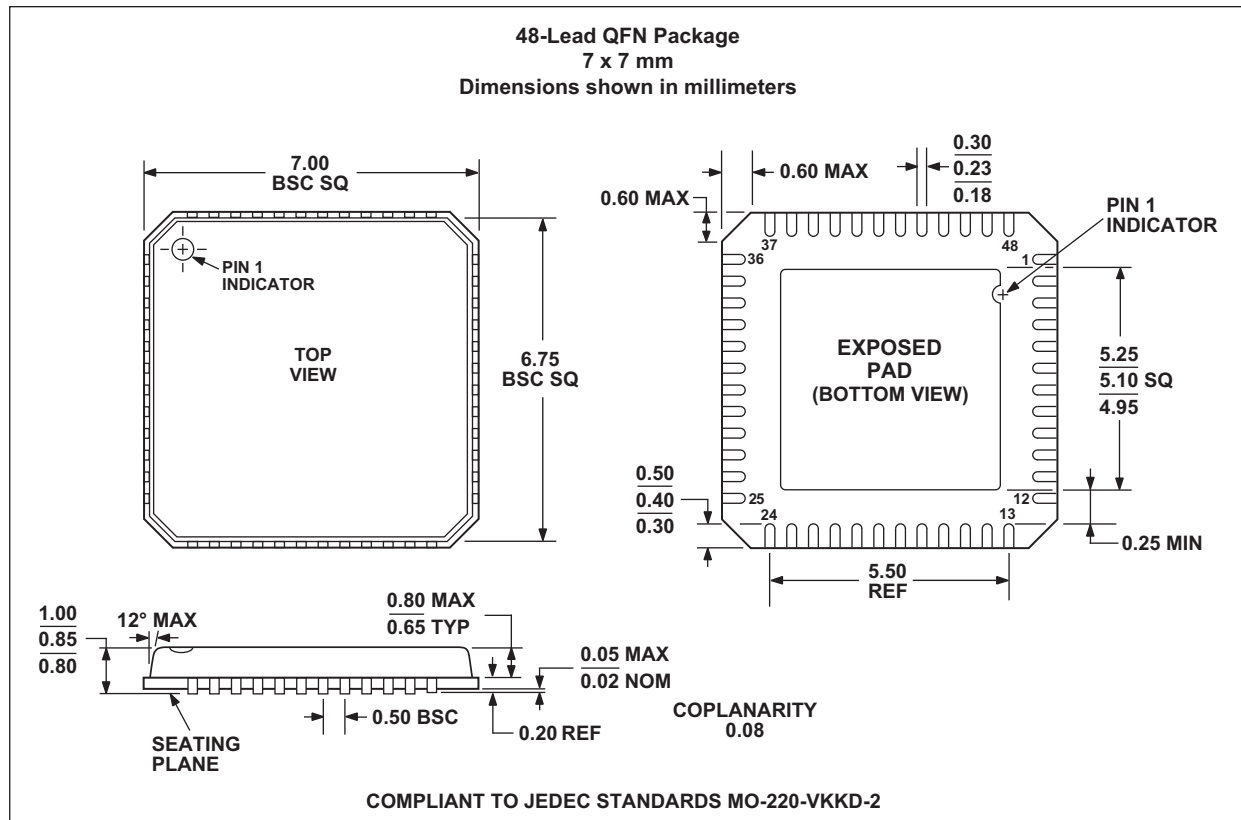
Figure 5. Package Dimensions
