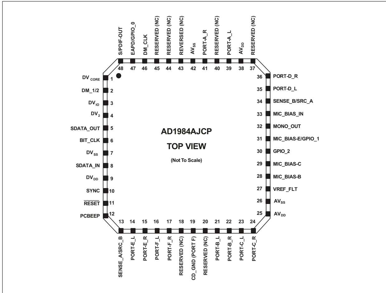
Figure 1. AD1984A Pinout
