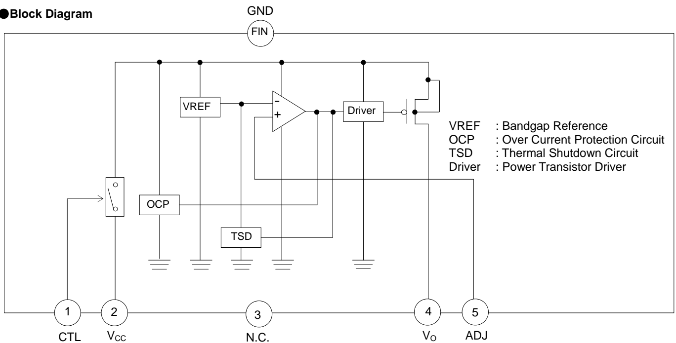
Figure 3. Block diagram
