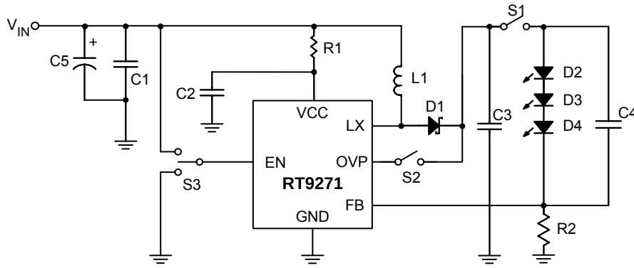
EVB Circuit
