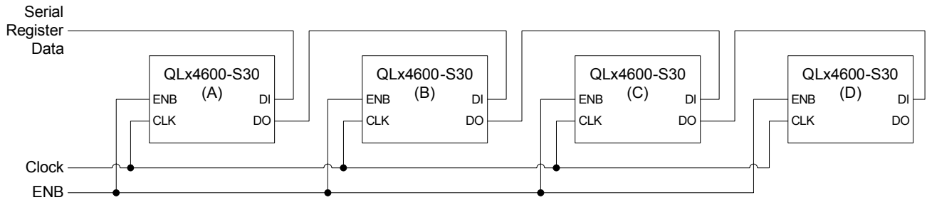
FIGURE 30. SERIAL BUS PROGRAMMING MULTIPLE QLx4600-S30 DEVICES USING DI/DO CARRYOVER
