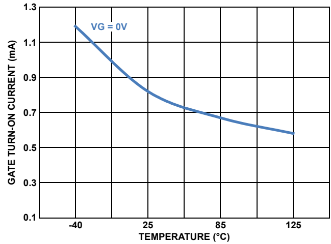
FIGURE 10. GATE TURN-ON CURRENT V_{th} = 12V
