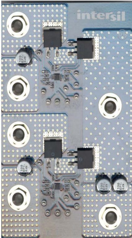
FIGURE 56. ISL6146AEVAL1Z
