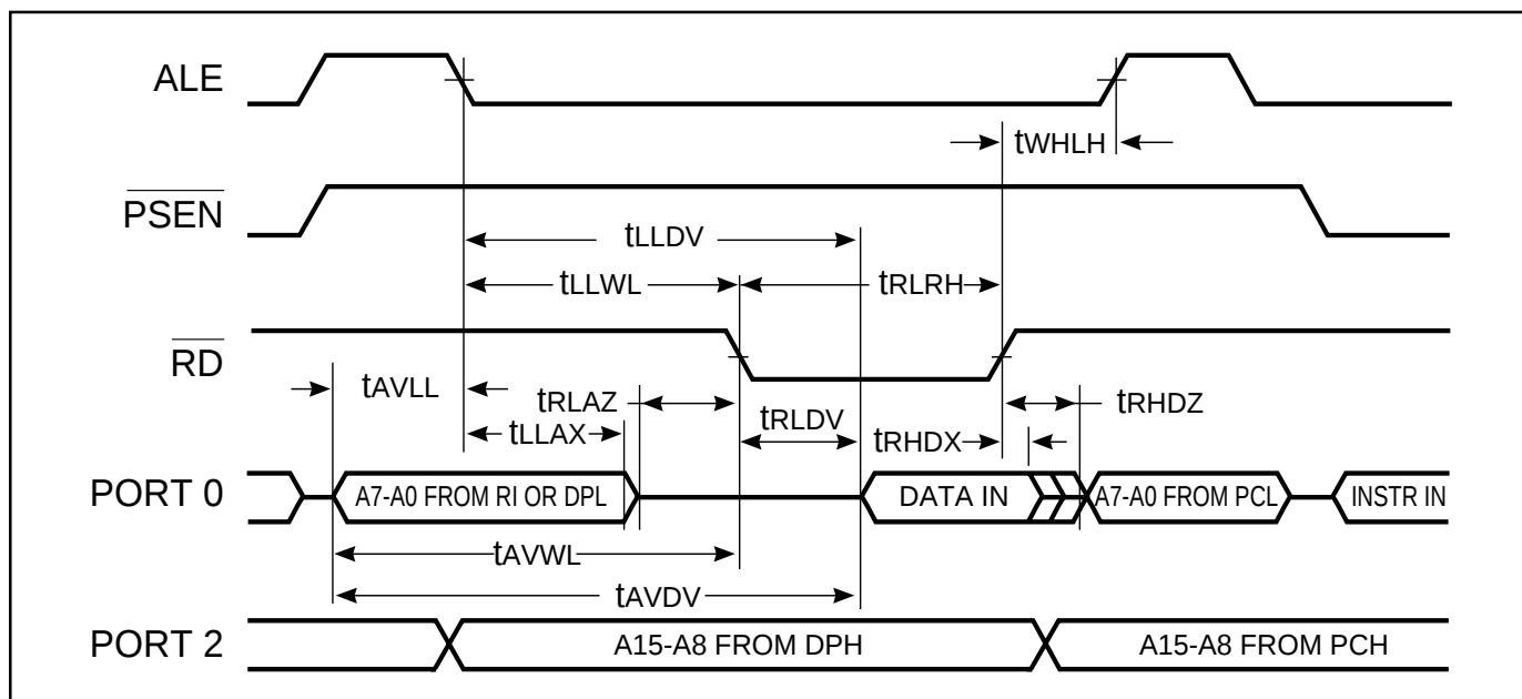
Figure 33. External Data Memory Read Cycle
