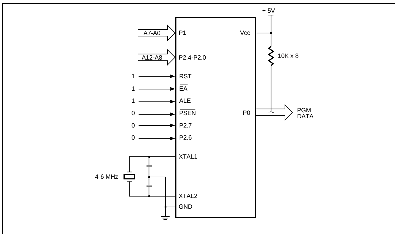
Figure 27. ROM Verification
