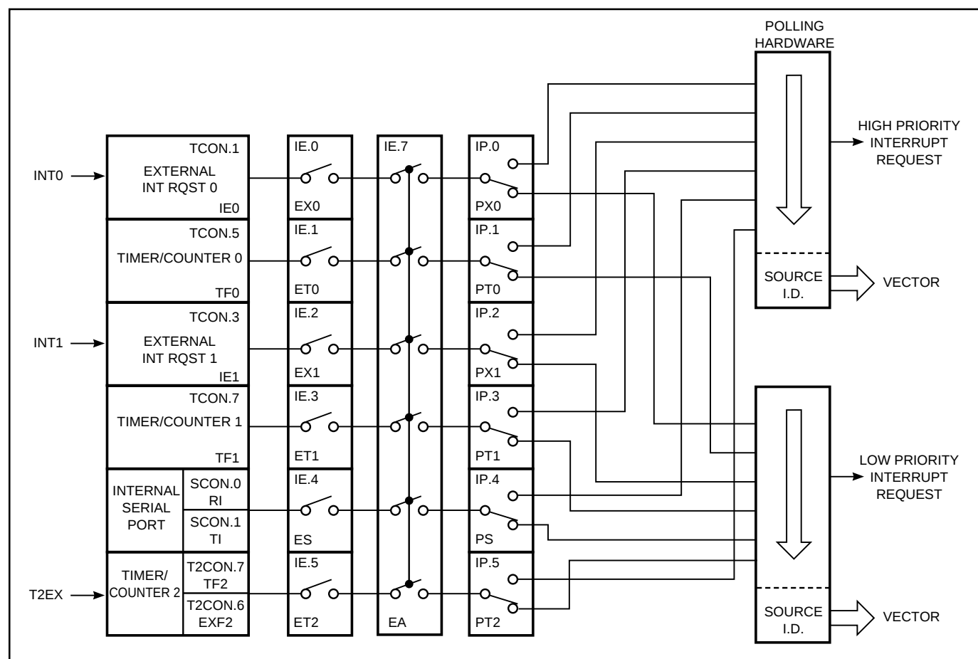
Figure 19. Interrupt System
