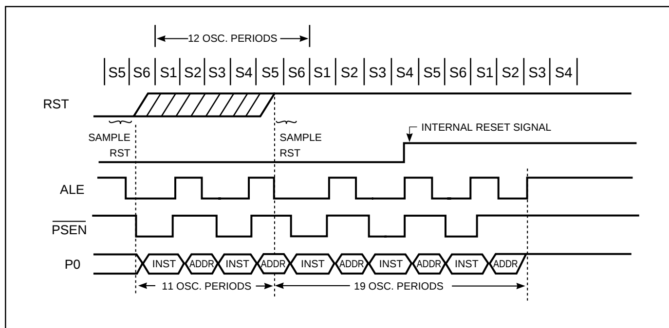
Figure 22. Reset Timing
