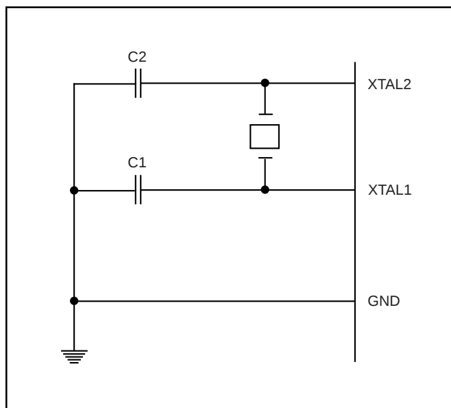
Figure 24. Oscillator Connections
