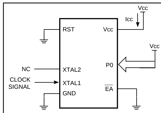
Figure 29. Idle Mode
