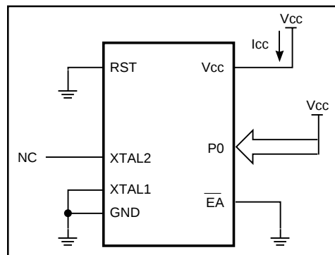
Figure 30. Power-down Mode
