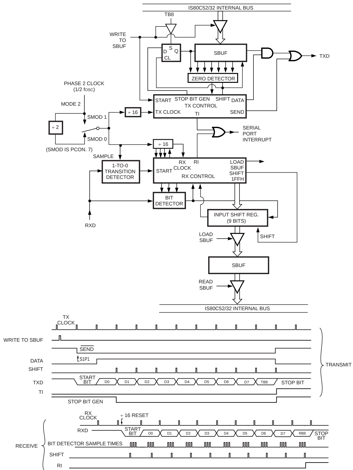
Figure 17. Serial Port Mode 2
