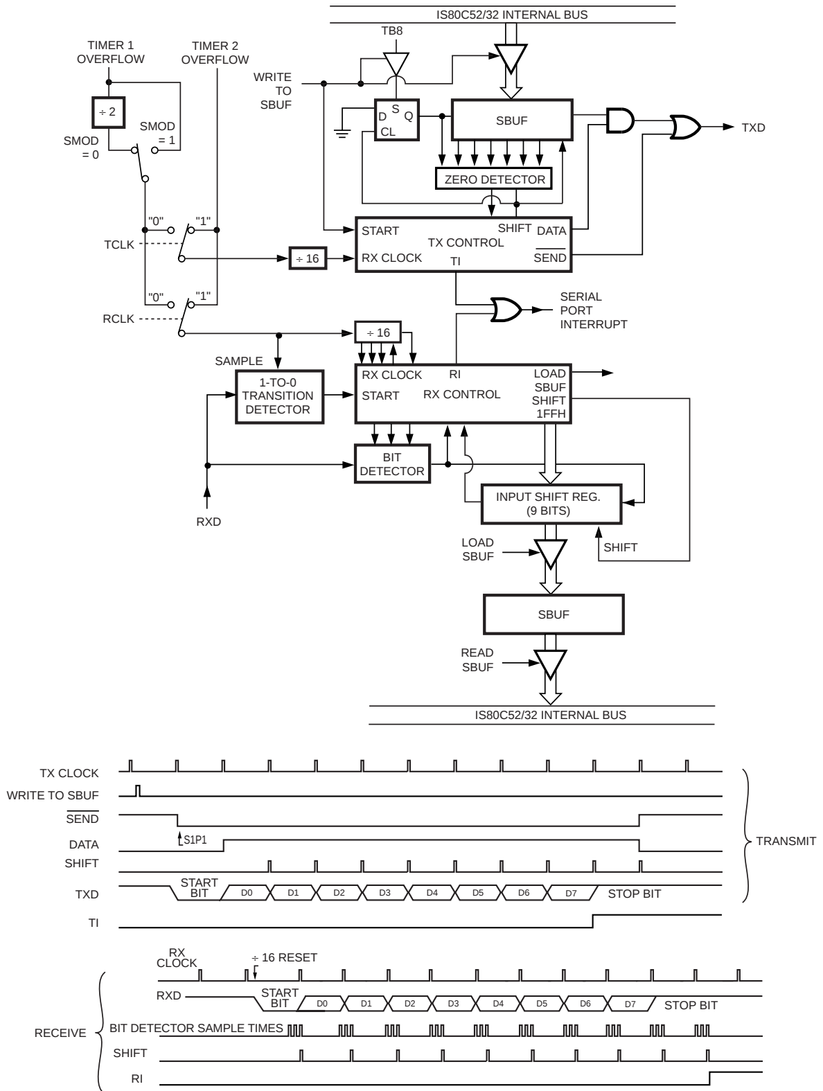
Figure 16. Serial Port Mode 1
