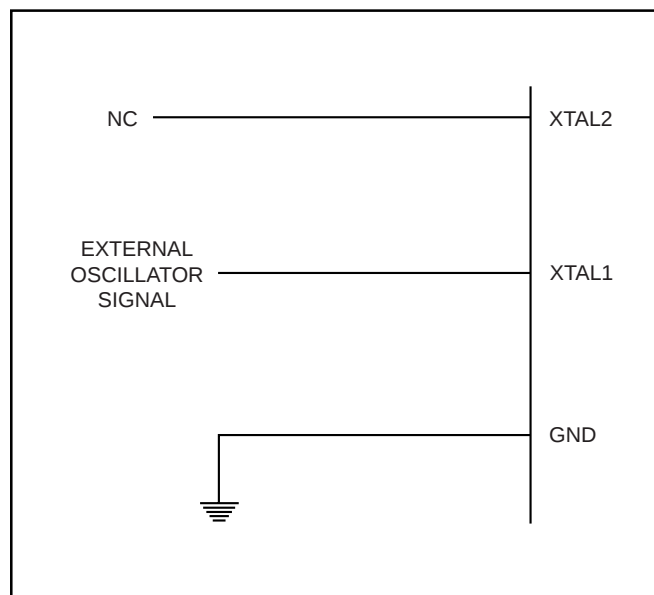
Figure 25. External Clock Drive Configuration
