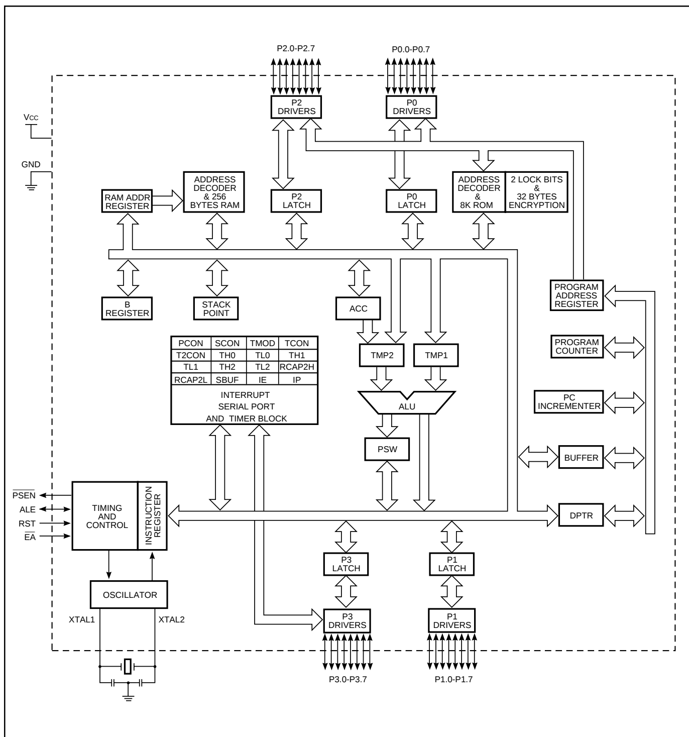
Figure 4. IS80C52/32 Block Diagram
