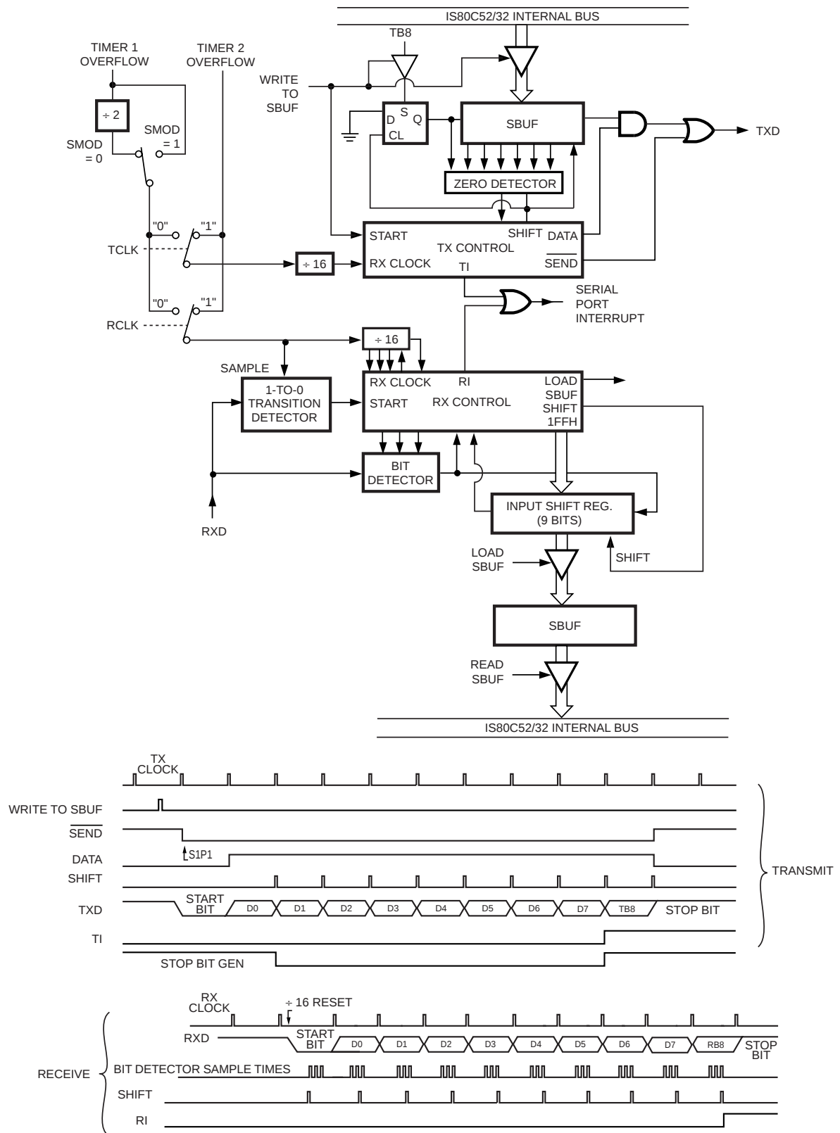
Figure 18. Serial Port Mode 3
