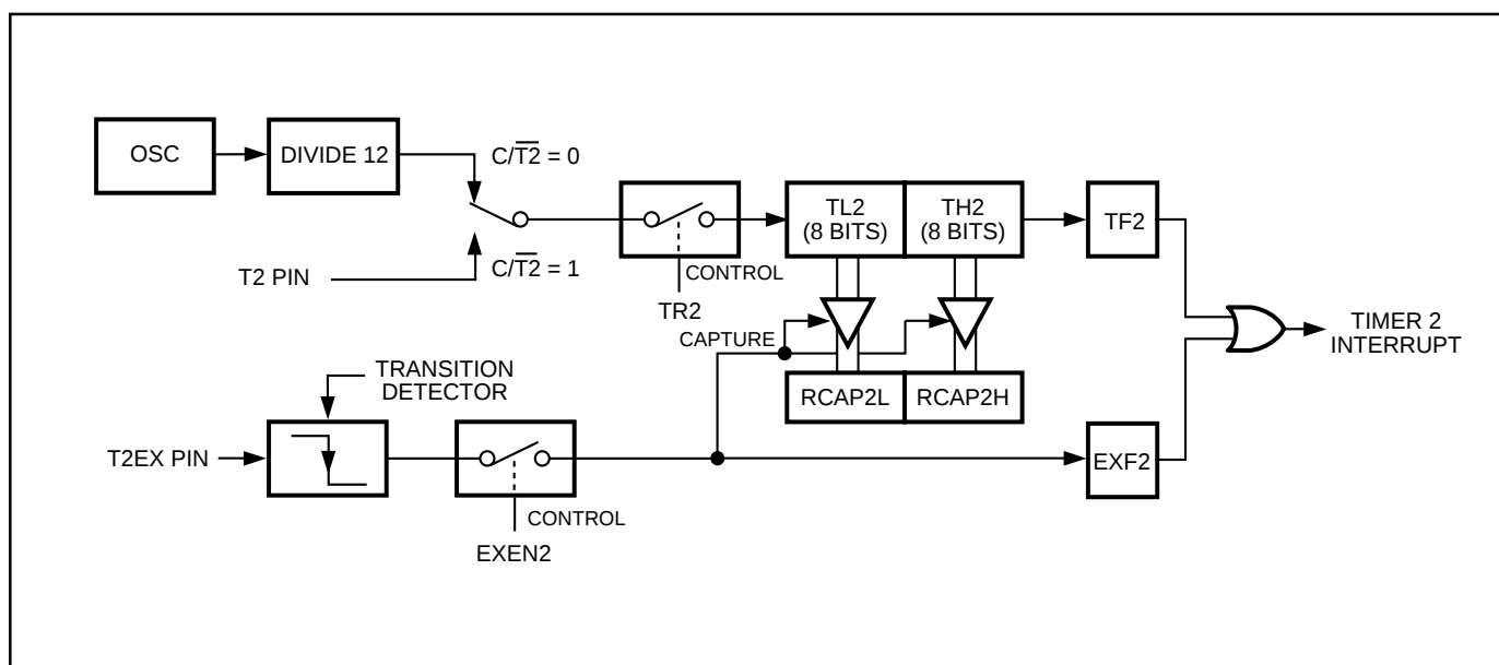
Figure 12. Timer 2 In Capture Mode
