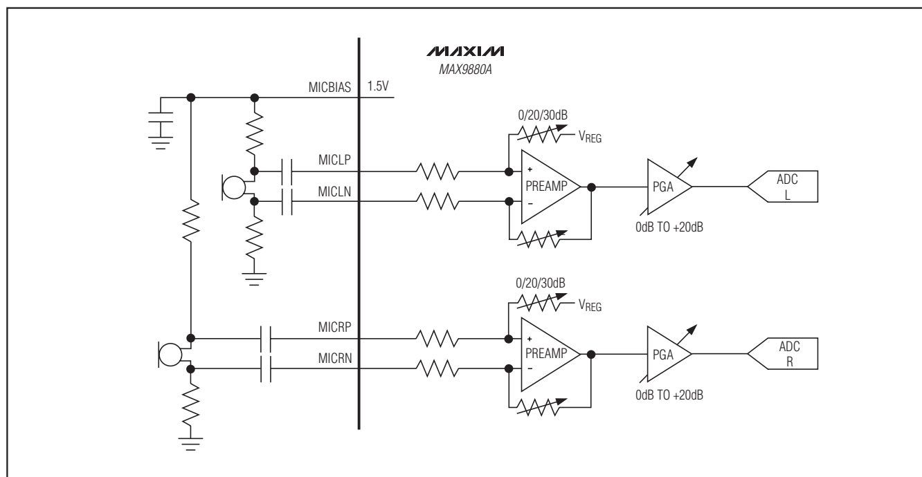
Figure 6. Microphone Input Block Diagram
