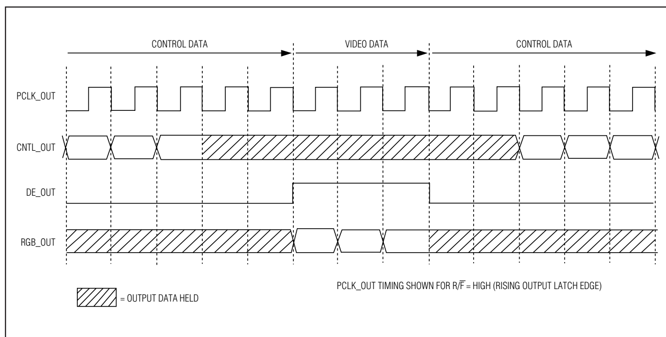
Figure 13. Output Timing
