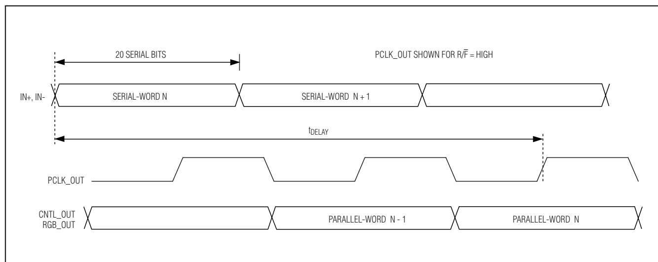
Figure 6. Deserializer Delay
