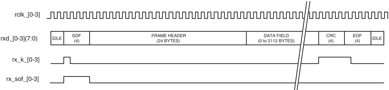
Figure 6-7. Fibre Channel Receive FPGA Interface Signals
