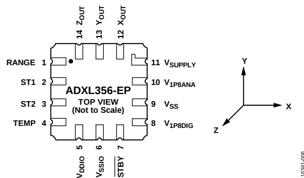
Figure 2. Pin Configuration
