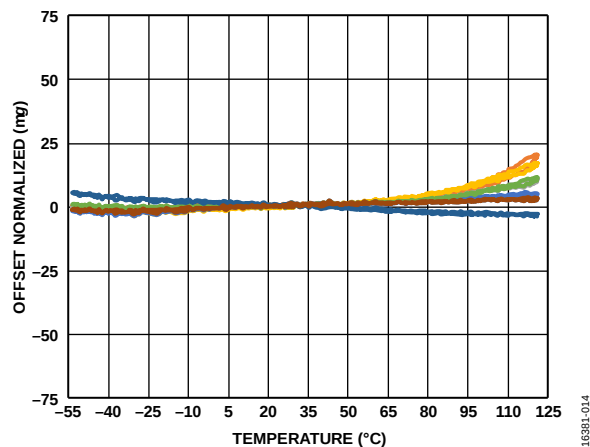
Figure 3. X-Axis Zero g Offset Normalized Relative to 25°C vs. Temperature for Multiple Devices
