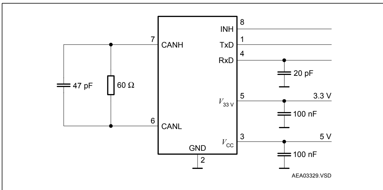
Figure 8 Test Circuit for Dynamic Characteristics (GV33 Version)
