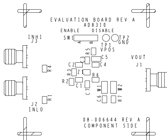
Figure 40. Component Side Silkscreen of Evaluation Board
