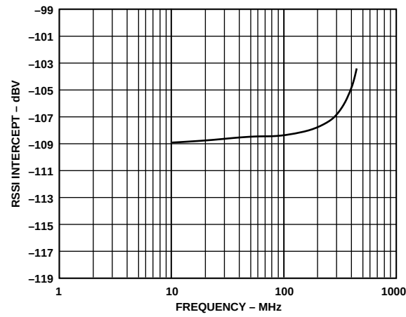
Figure 16. RSSI Intercept vs. Frequency
