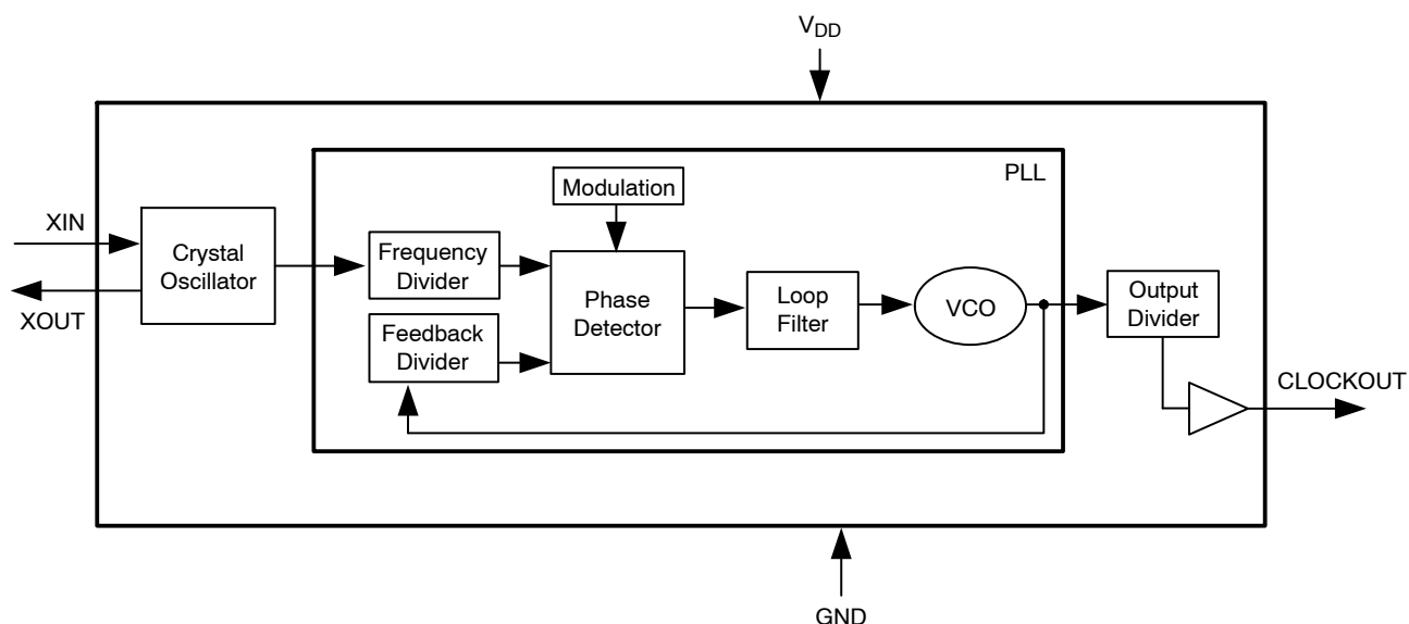
Figure 1. Block Diagram
