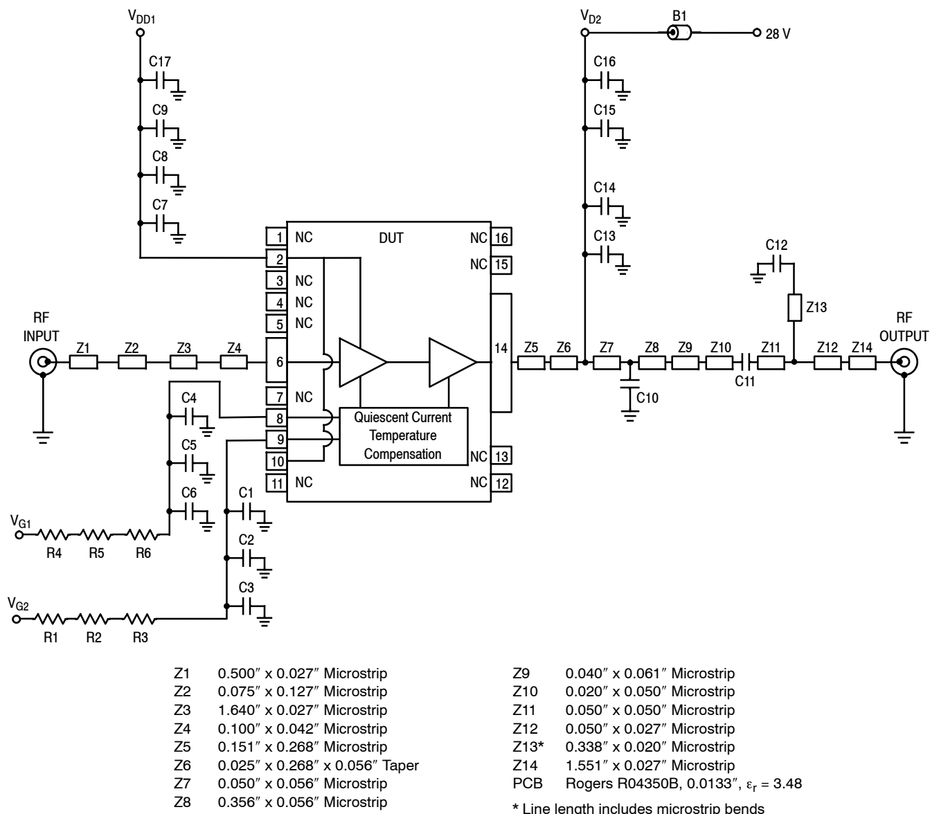
Figure 3. MMRF2004NBR1 Test Circuit Schematic
