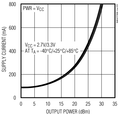
MAX2266 SUPPLY CURRENT vs. OUTPUT POWER
