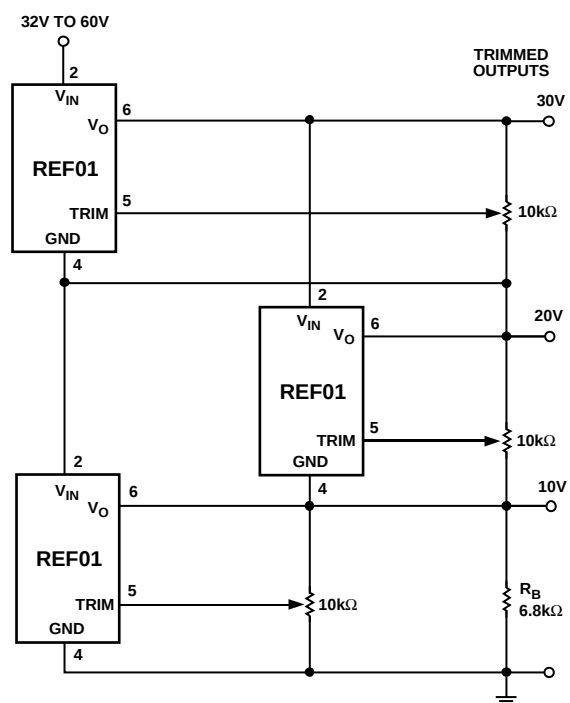
Figure 21. Reference Stack
