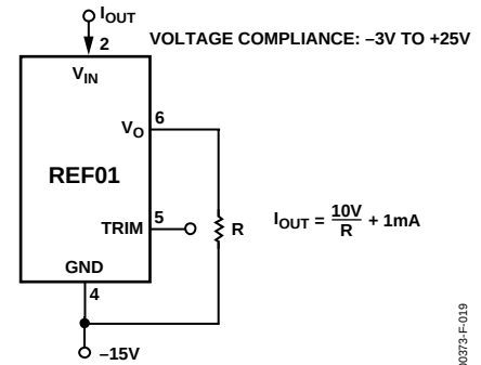
Figure 19. Current Sink
