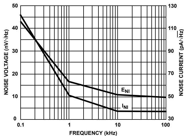
FIGURE 38. INPUT NOISE CHARACTERISTICS
