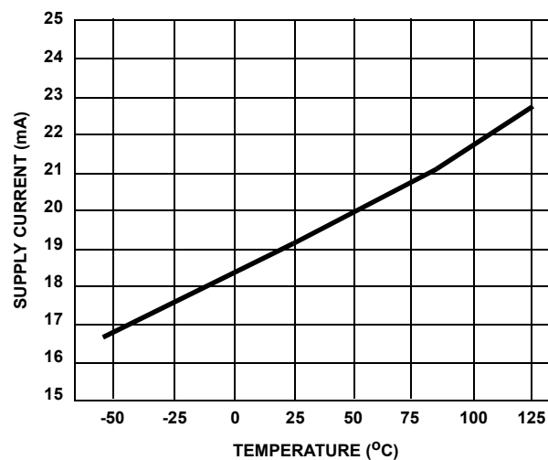
FIGURE 36. SUPPLY CURRENT vs TEMPERATURE
