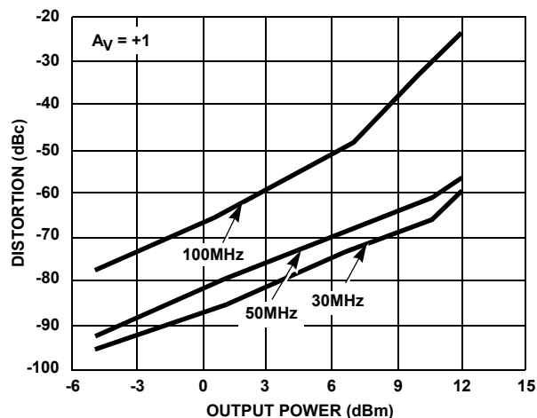
FIGURE 28. 3rd HARMONIC DISTORTION vs P_{\text{OUT}}
