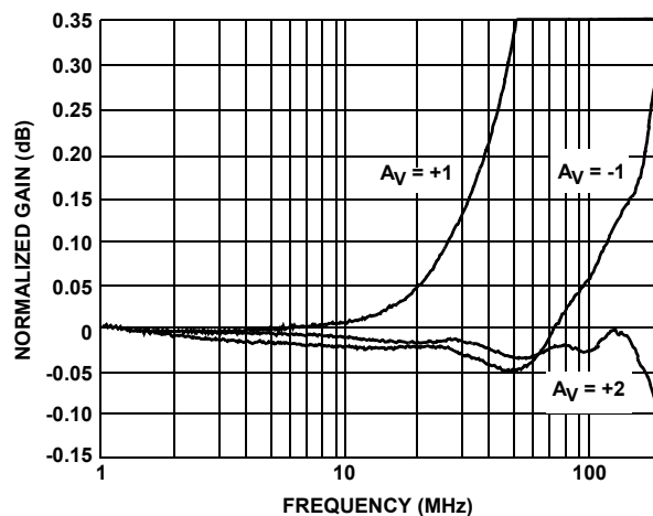
FIGURE 18. GAIN FLATNESS
