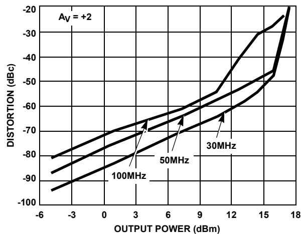
FIGURE 26. 3rd HARMONIC DISTORTION vs P_{\text{OUT}}
