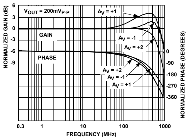
FIGURE 9. FREQUENCY RESPONSE
