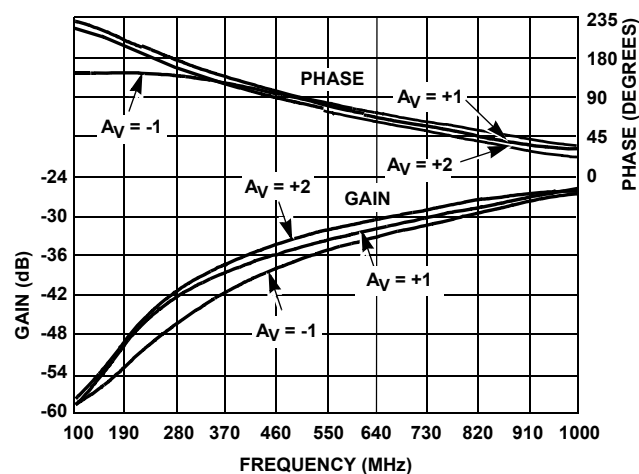
FIGURE 22. HIGH FREQUENCY REVERSE ISOLATION ( S_{12} )
