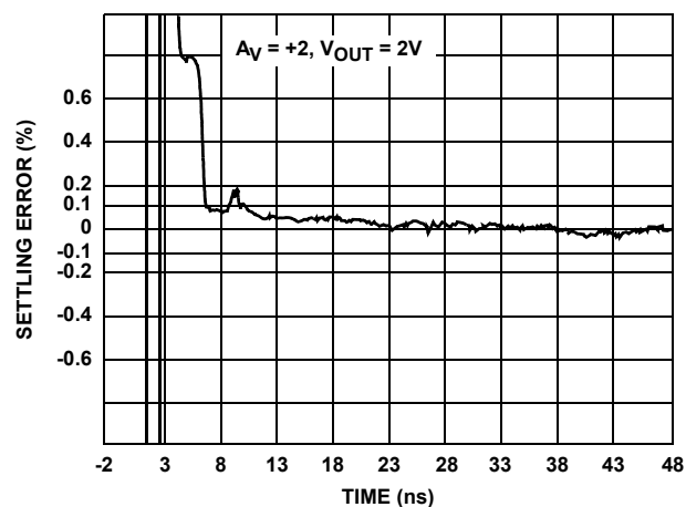
FIGURE 20. SETTLING RESPONSE
